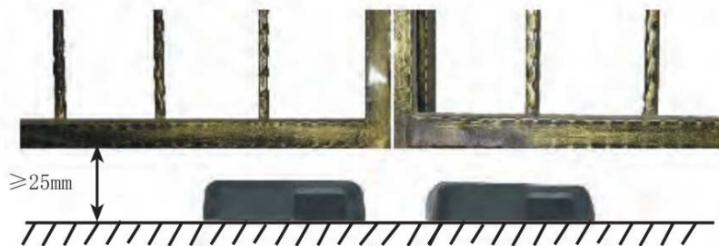
Fig.4 Heights of Gate Frame and Stop Irons
